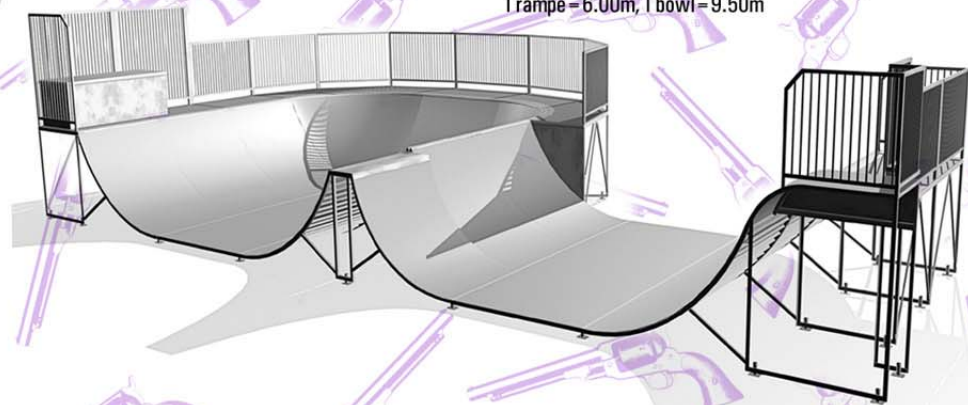
Exemple de Combo Spine & Bowl h rampe & bowl=1.50m, h canyon=2.00m, h sub box=2.50m l rampe=6.00m, l bowl=9.50m
