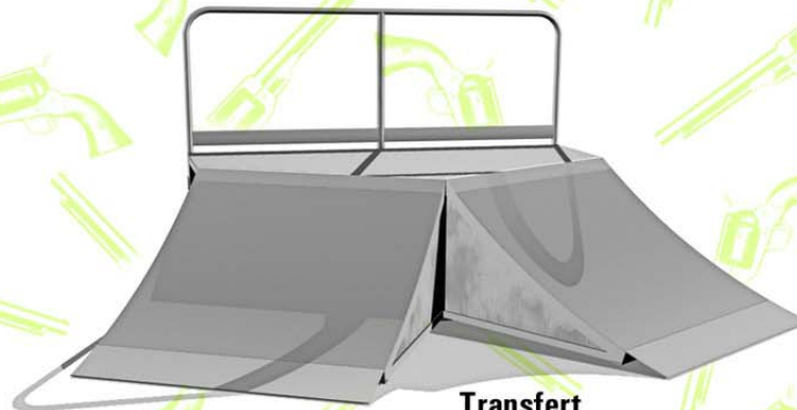
Transfert h = 0.80m, l courbes = 1.50m
